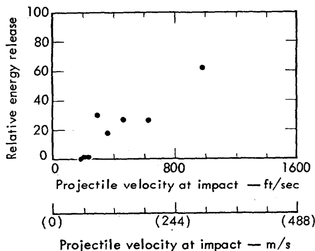
Fig 5 Susan Test: Octol 75/25. Conversion factor: 1 ft/sec = 3.048 \times 10^{-1} m/s
